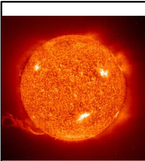
soleil
