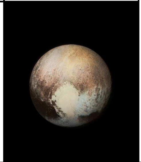
pluton
